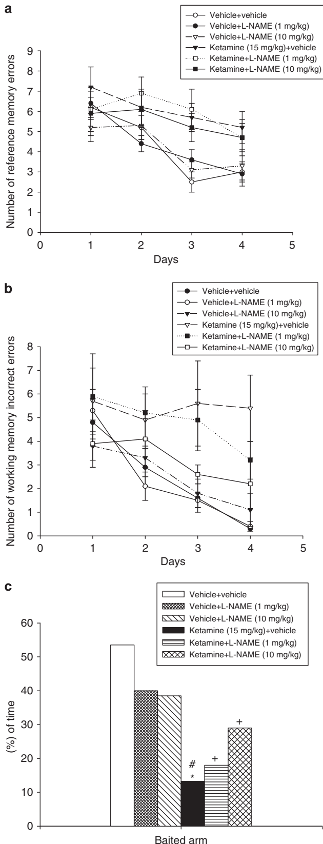
Figure 4 Radial water maze task. Vehicle, ketamine, and L-NAME were injected i.p., every day 40 and 60 min, respectively, before testing. (a) Spatial reference memory. Results are expressed as mean ± SEM. Number of errors cumulating over days by different groups of rats. (b) Spatial working memory. Results are expressed as mean ± SEM. Number of errors cumulating over days by different groups of rats. (c) Percentage of total time spent in the previously reinforced arm of the radial water maze by different groups of rats. Results are expressed as medians. * p < 0.05 vs the vehicle + vehicle-treated animals; + p < 0.05 vs the respective control populations; # p < 0.05 vs ketamine + L-NAME 10 mg/kg-treated rats.
