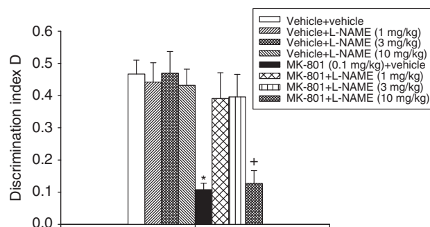
Figure 1 Novel object recognition task. Vehicle, MK-801, and L-NAME were injected i.p., just after T1. The 3-h ITI was used. Results are expressed as mean \pm SEM. Discrimination index D performance expressed by different groups of rats during T2. * p < 0.05 vs all the other groups (except the MK-801 + L-NAME 10 mg/kg group); + p < 0.05 vs all the other groups (except the MK-801 + vehicle group).
